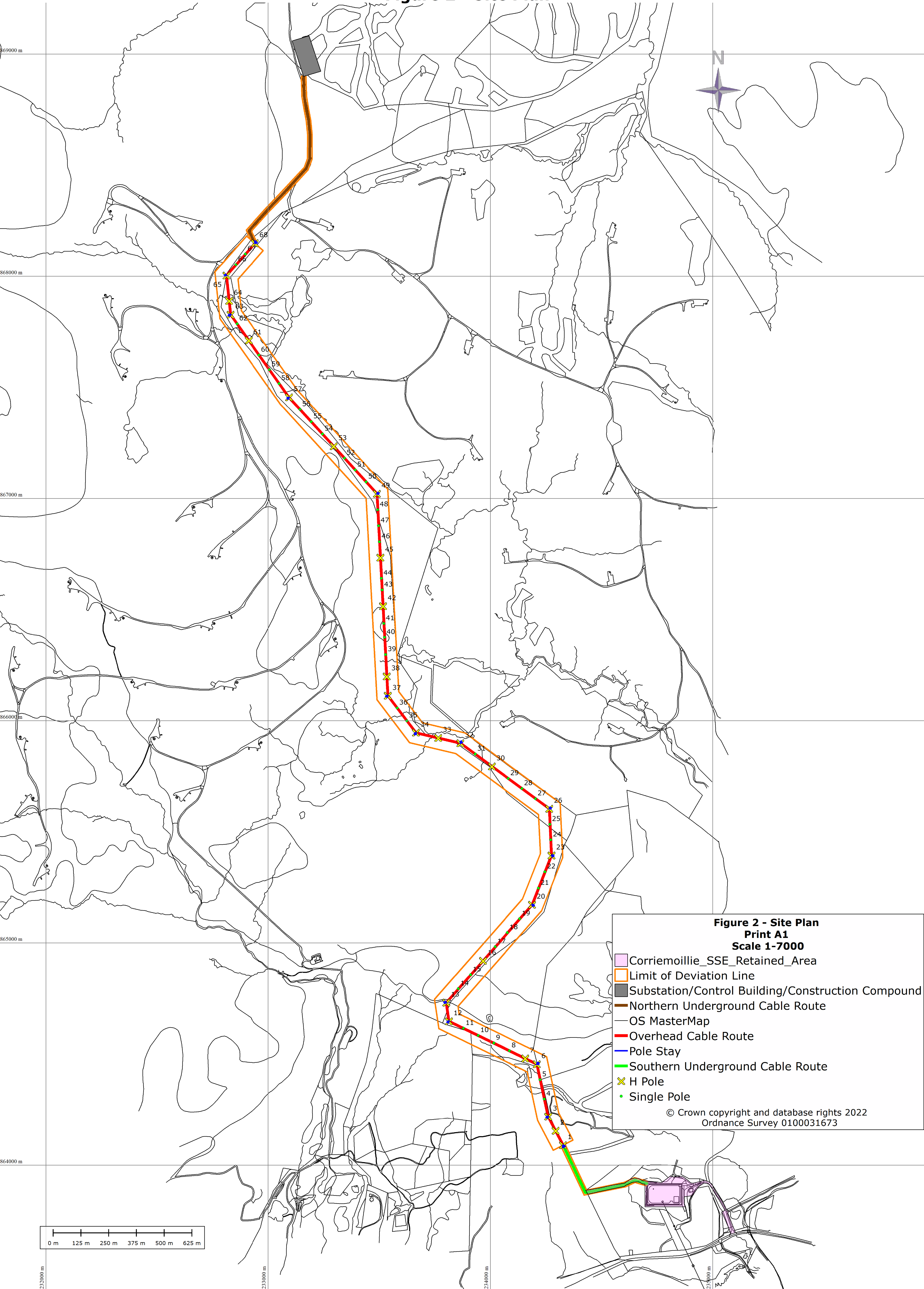
Figure 2 - Site Plan
