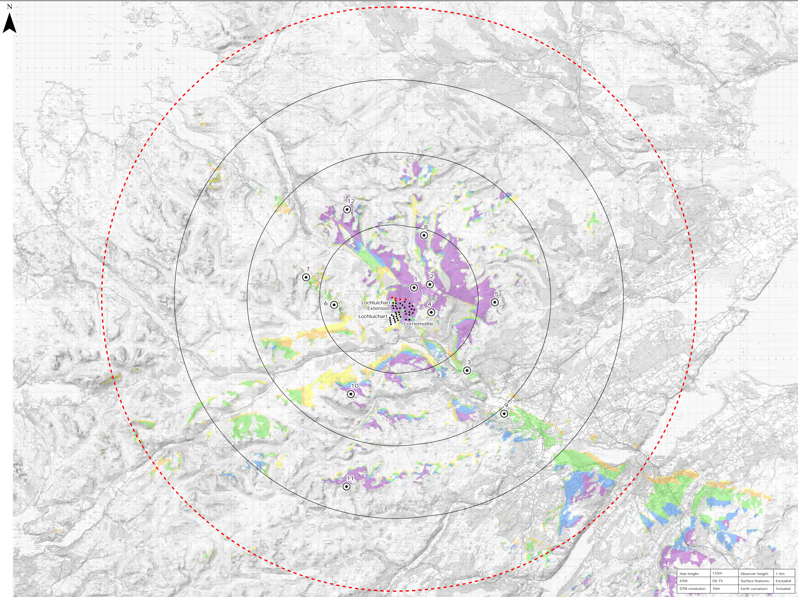
Figure 8.7a: Hub Height ZTV with Viewpoints (40km)
