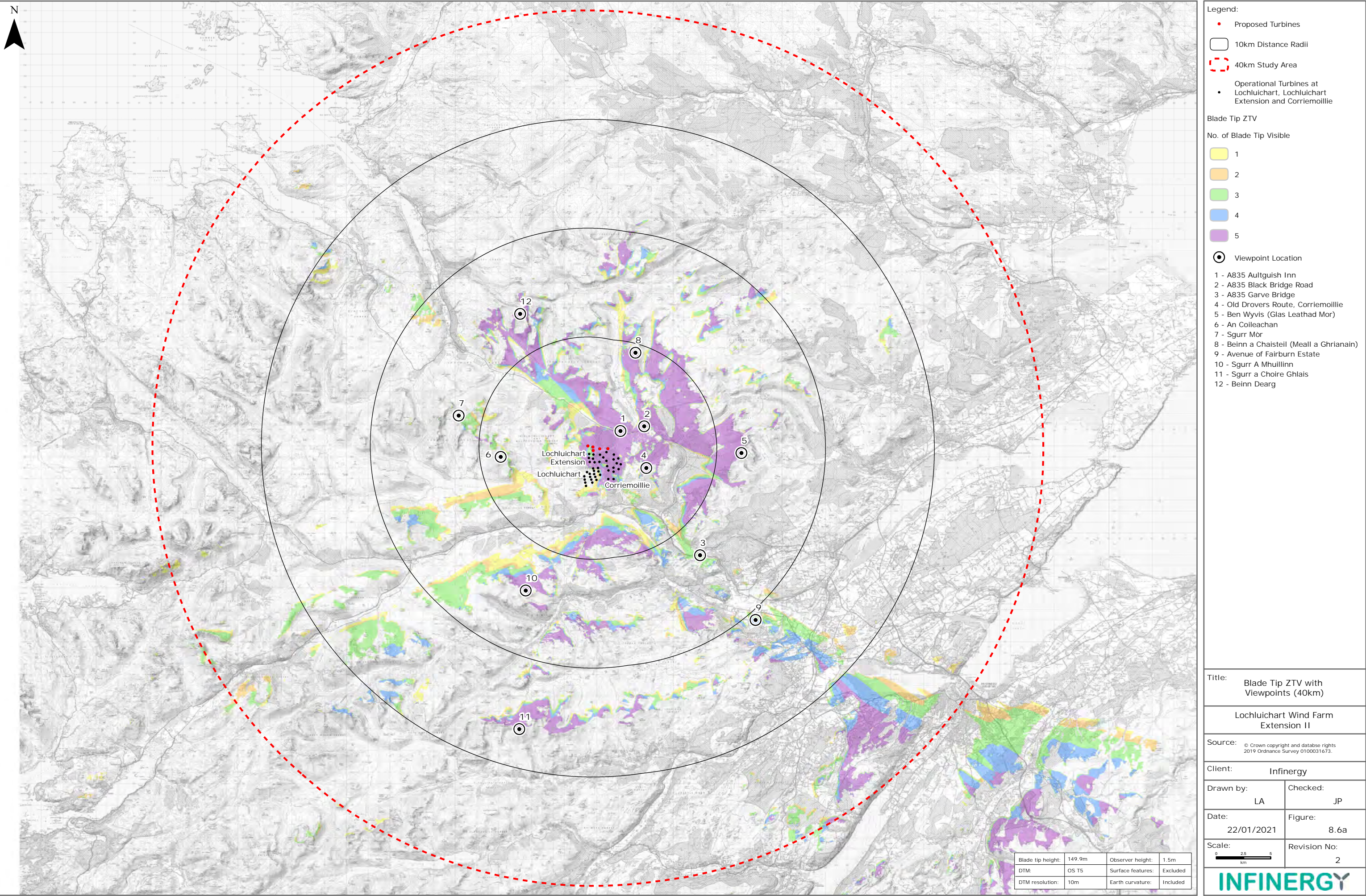
Figure 8.6a: Blade Tip ZTV with Viewpoints (40km)
