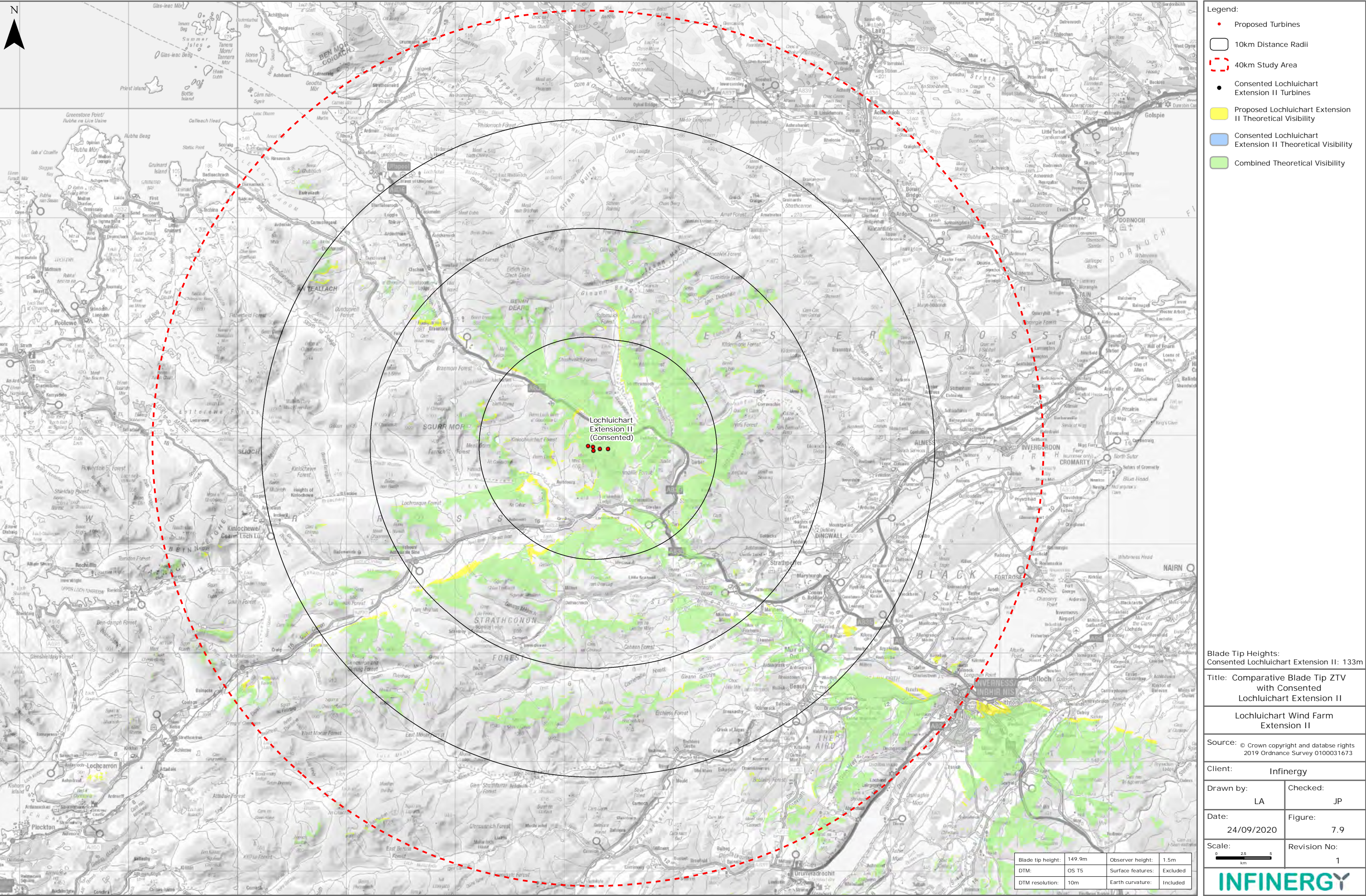
Figure 7.9: Comparative Blade Tip ZTV with Consented Lochluichart Extension II
