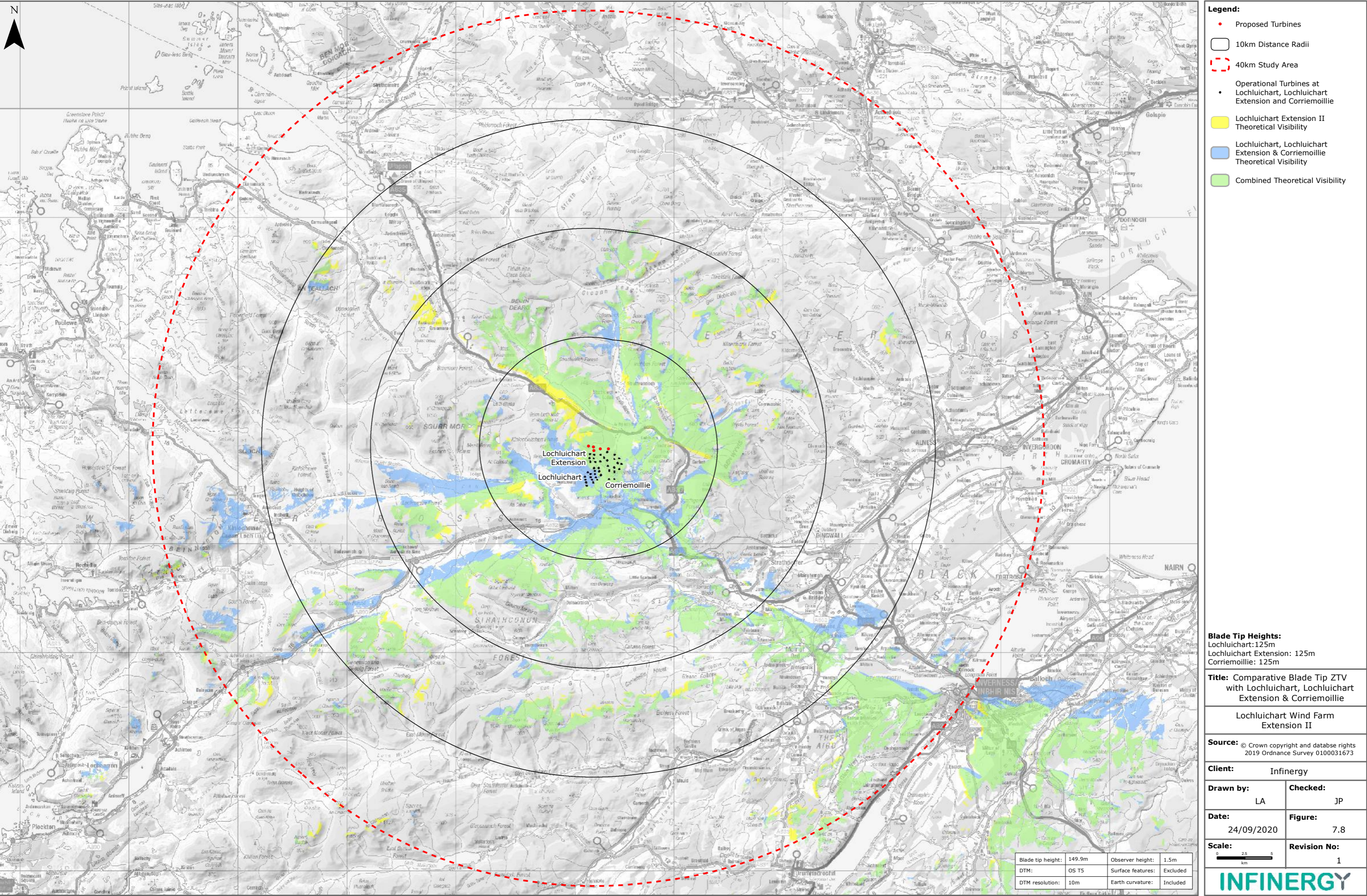
Figure 7.8: Comparative Blade Tip ZTV with Lochluichart, Lochluichart Extension & Corriemoillie
