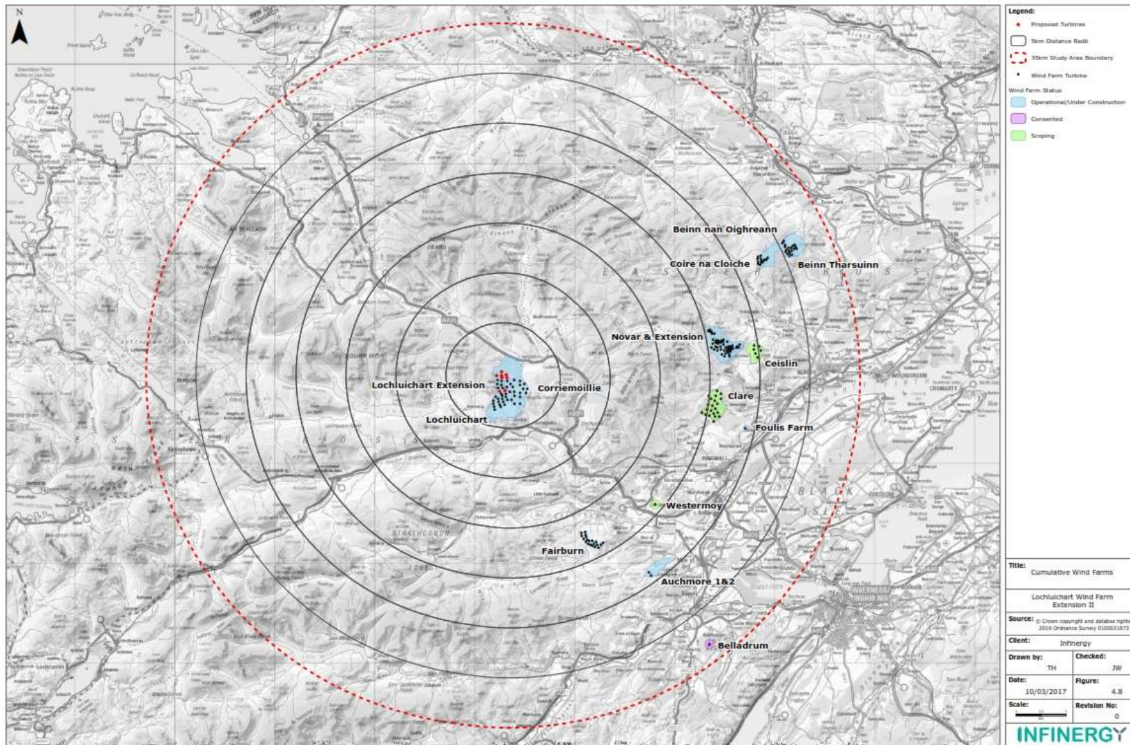
Figure 4.8: Cumulative Wind Farms
