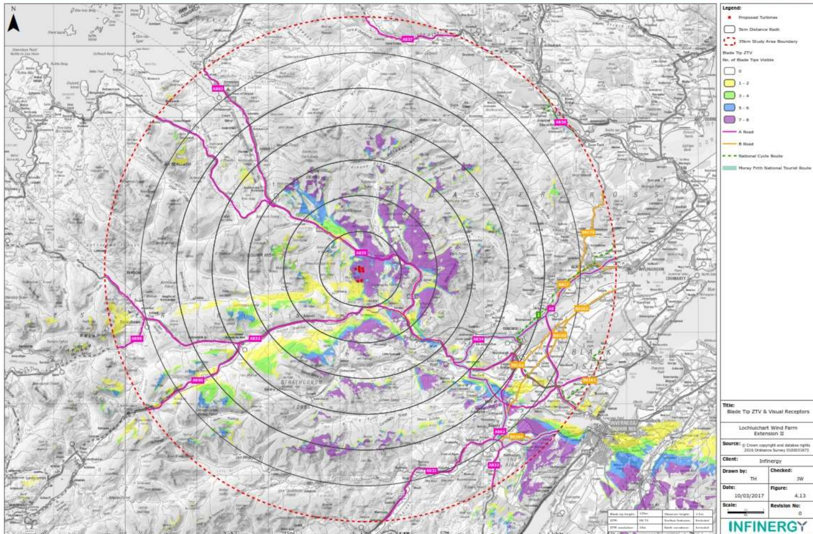
Figure 4.13: Blade Tip ZTV & Visual Receptors
