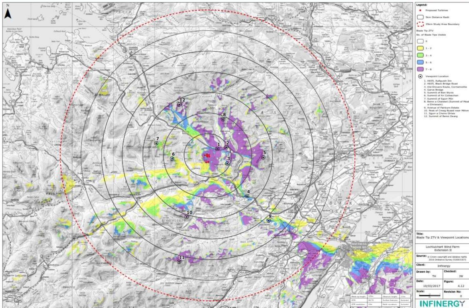
Figure 4.12: Blade Tip ZTV & Viewpoint Locations
