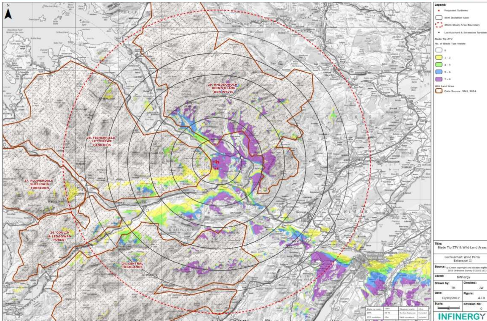
Figure 4.10: Blade Tip ZTV & Wild Land Areas
