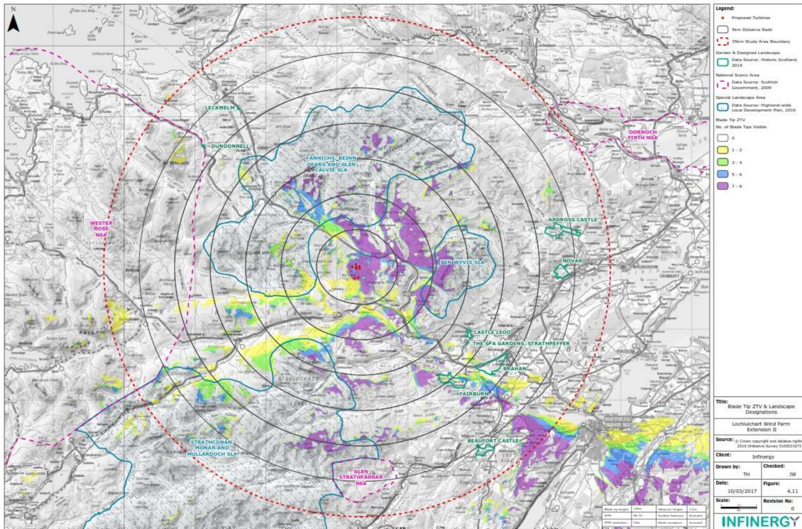
Figure 4.11: Blade Tip ZTV & Landscape Designations
