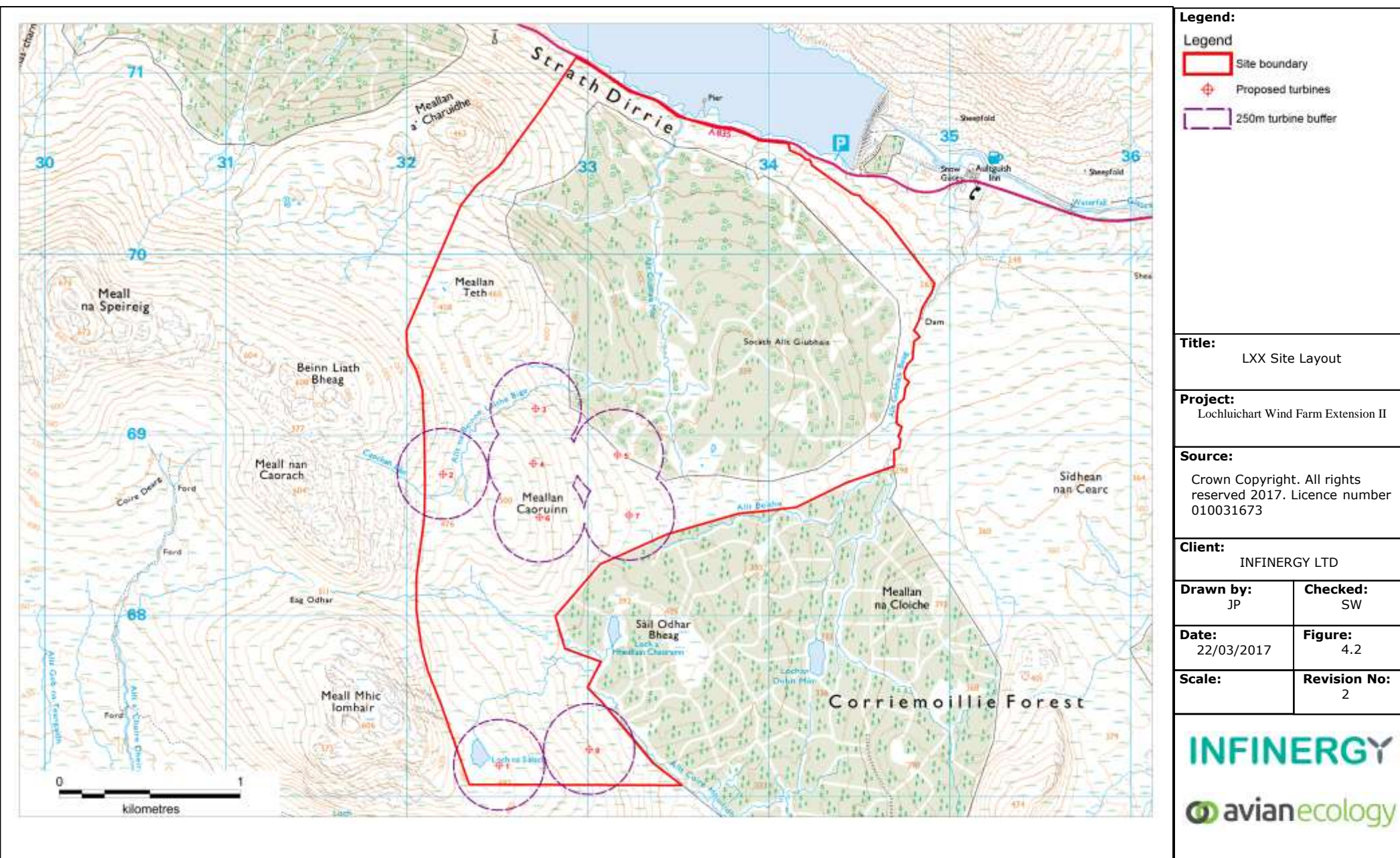
Figure 4.2: LXX Site Layout
