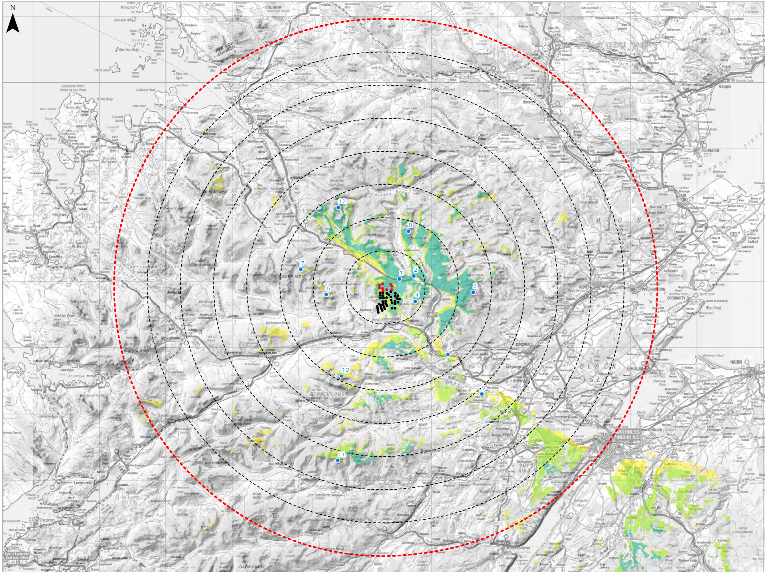
Figure 9.7a: Hub Height ZTV with Viewpoints (40km)
